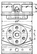
Figs. 3352-3356. Center Plate of Pony Truck for Mogul (2-6-0) Locomotive. American Locomotive Co.
